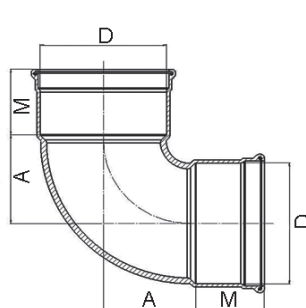
PVC Bocht 90mm 2 x mof 90°
