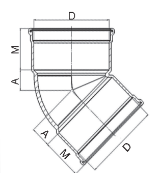
PVC Bocht 90mm 2 x mof 45°
