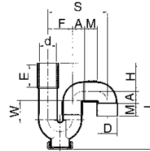
Universele sifons
