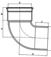
Bocht 90° manchetterverbinding mof/spie
