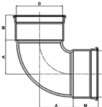
Bocht 90° manchetterverbinding mof/mof
