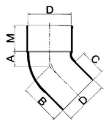
Bochten 22°30' lijmvverbinding mof/spie
