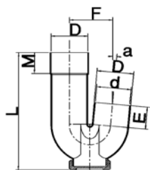
HWA sifon lijmvverbinding
