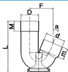
HWA sifon lijmvverbinding
