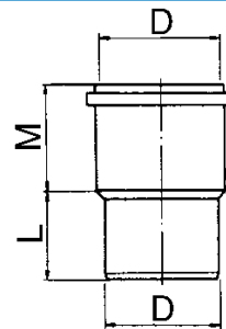
Inbouwmof manchetverbinding mof/spie
