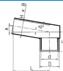
Stadsuitloop 6 x 8 cm of 6 x 10 cm (op buis 70 of 80)
