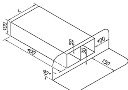
Vacurain noodoverlaten 90°
