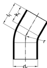
Bocht 30° (segment)
