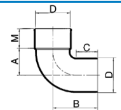
Bochten 87°30' lijmverbinding mof/spie
