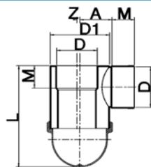
Riolsifon lijmvverbinding
