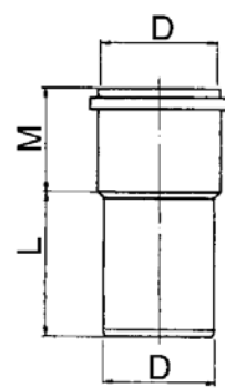
Verlengde inbouwmof manchetverbinding mof/spie
